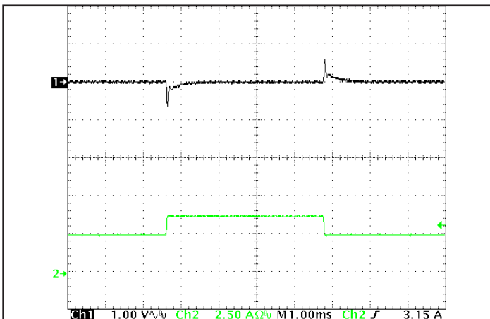
Figure 5: Output voltage response to step-change in load current (70% -100% -70% of I out (max); dI/dt = 0.1 A/μs). Load cap: 15 μF tantalum cap and 1 μF ceramic cap. Ch 1: V out , Ch 2: I out .
