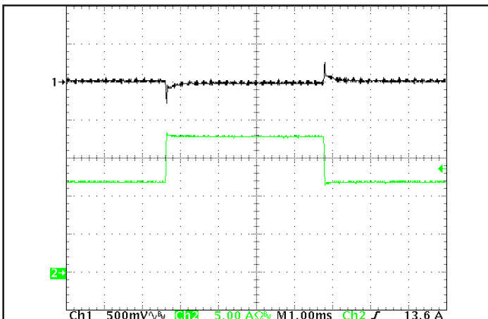
Figure 5: Output voltage response to step-change in load current (70 % -100 % -70 % of Iout(max); dI/dt = 0.1 A/μs). Load cap: 15 μF tantalum cap and 1 μF ceramic cap. Ch 1: Vout, Ch 2: Iout.
