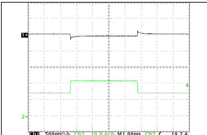
Figure 5: Output voltage response to step-change in load current (65% -100% -65% of I out (max); dI/dt = 0.1 A/μs). Load cap: 15 μF tantalum cap and 1 μF ceramic cap. Ch 1: V out , Ch 2: I out .
