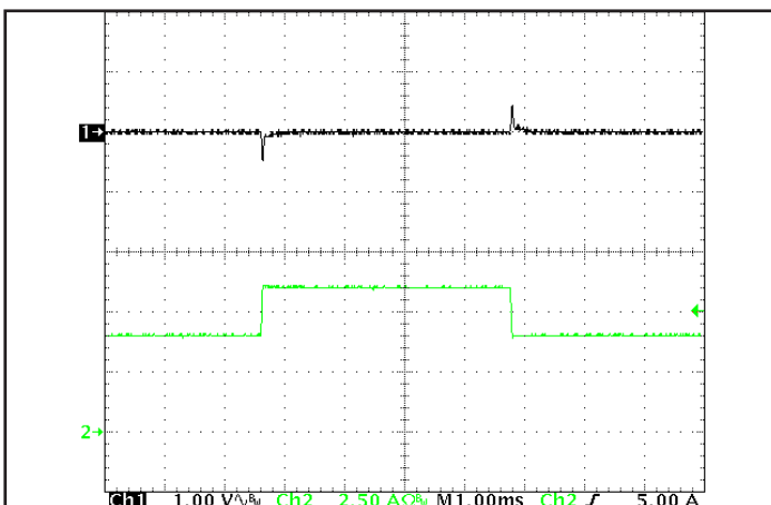
Figure 5: Output voltage response to step-change in load current (75% -100% -75% of I out (max); dI/dt = 0.1 A/μs). Load cap: 15 μF tantalum cap and 1 μF ceramic cap. Ch 1: V out , Ch 2: I out .
